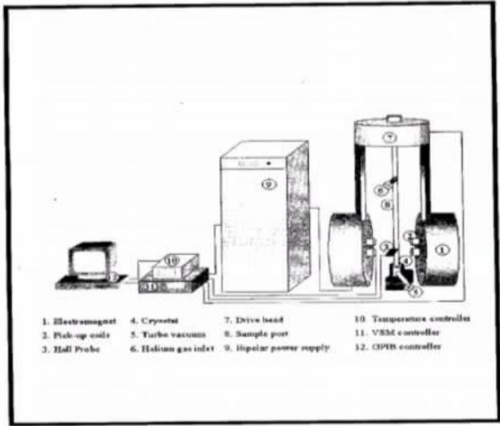
Fig. 3. Vibrating sample magnetometer.
